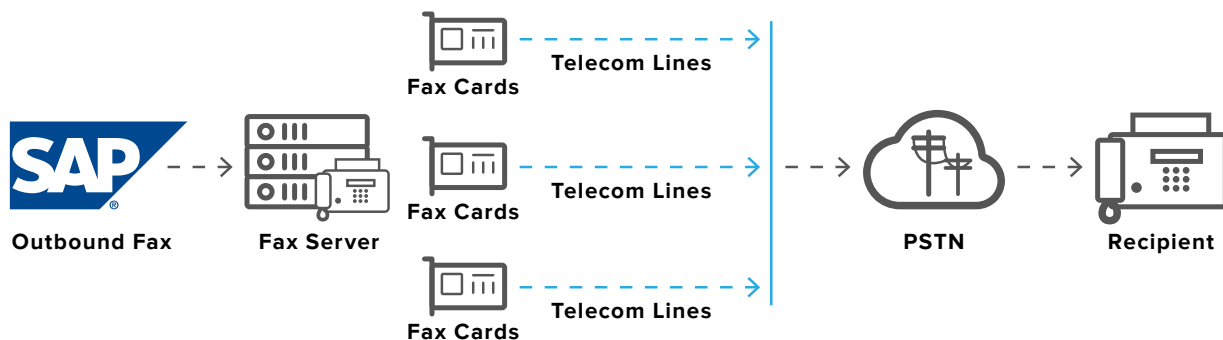
Figure A: Typical hardware-based fax solution built for high-volume traffic
